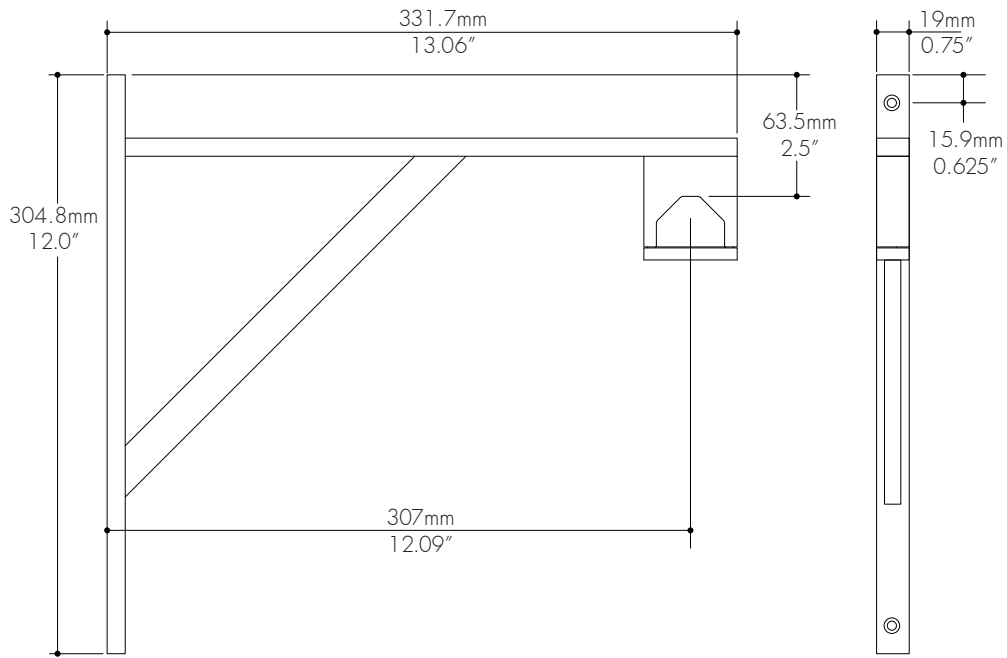
scale- 1:4 wall mount bracket
