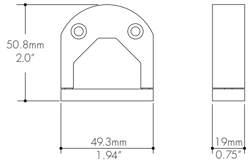
scale- 1:2 wall mount
